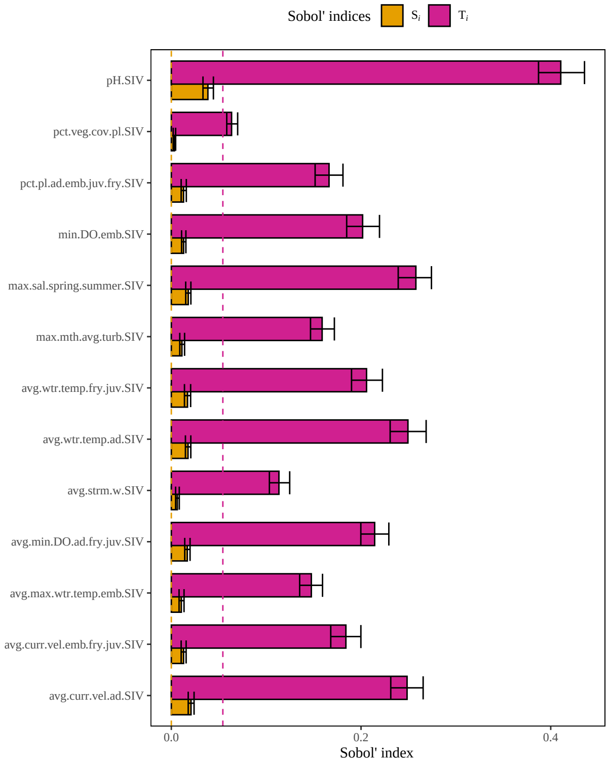
Figure 7. Results of a sensitivity analysis for the smallmouthbuffaloRiv model based on a multiplicative mean structure. Dashed lines represent baseline numerical approximation error for S_i and T_i ( i.e. , dummy variables).
